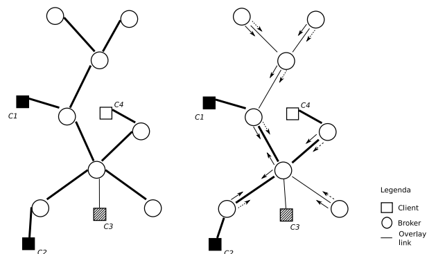
Figure 1: Routing on an acyclic overlay. Clients C1 and C2 are subscribed to the same “filled” filter, while client C3 is subscribed to a “dashed” filter. Where present, arrows represent the content of brokers’ routing tables, while thick lines represent the links followed by a message sent by client C4 , which matches the filled filter.
